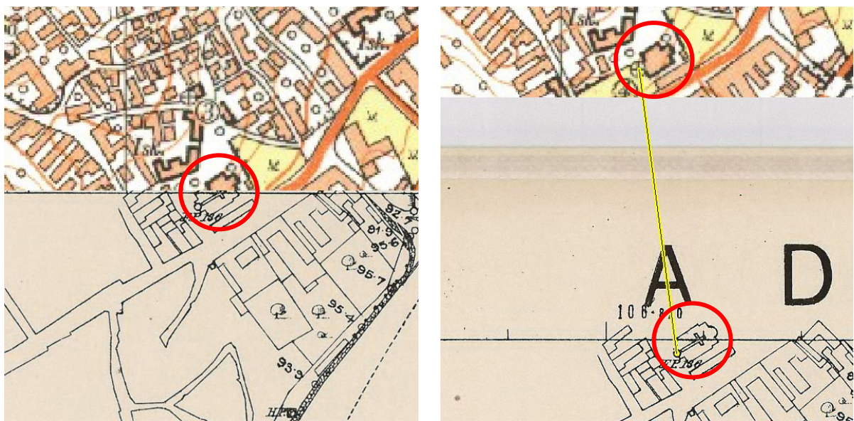
Figure 2: The error of the georeferenced map sheet: Cassini–Soldner projection (left) and stereographic projection (right)
